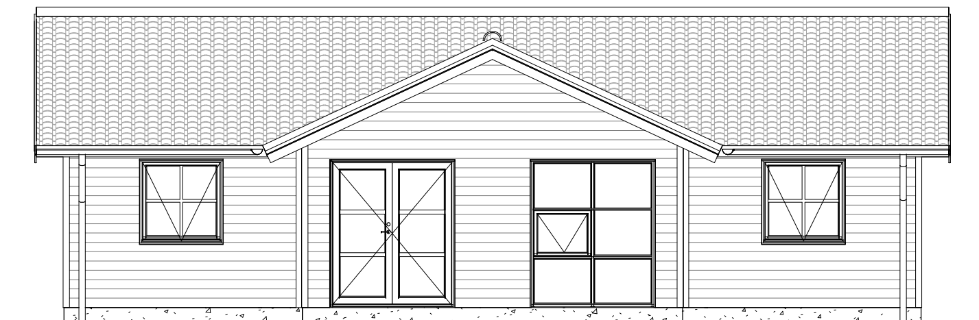
Facade 3
