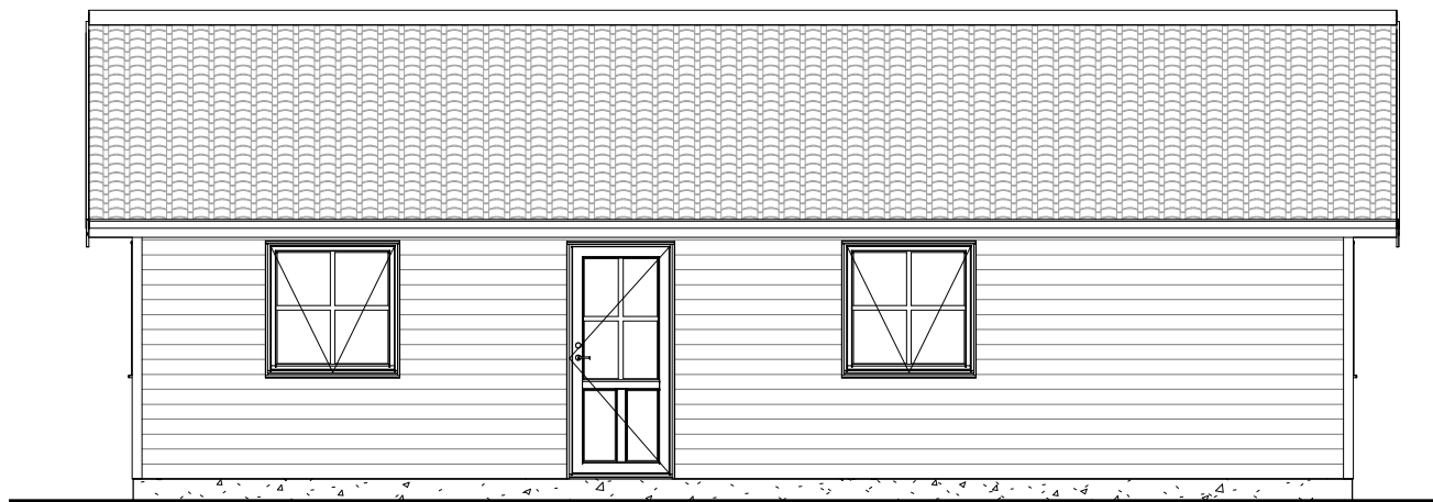
Facade 1
