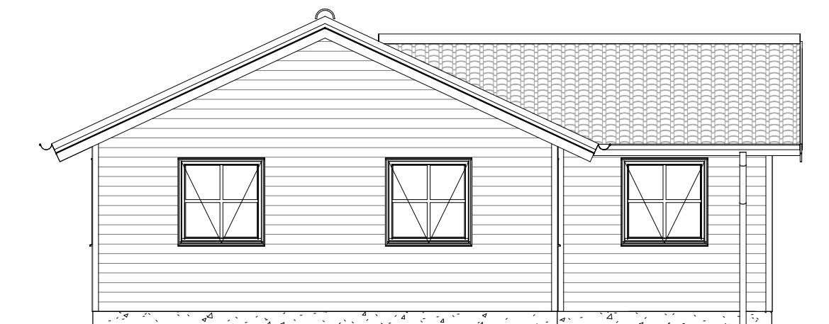
Facade 4
